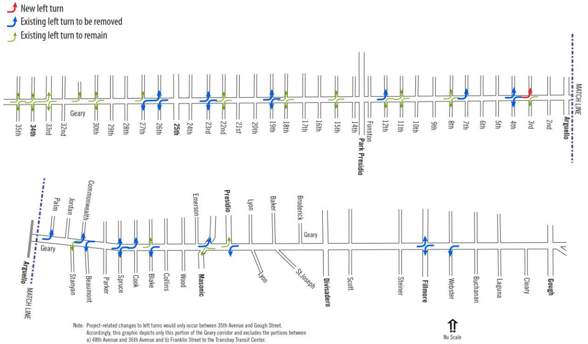
Figure 2-13 Figure 2-17 Proposed Left-Turn Locations for Alternative 3-Consolidated
