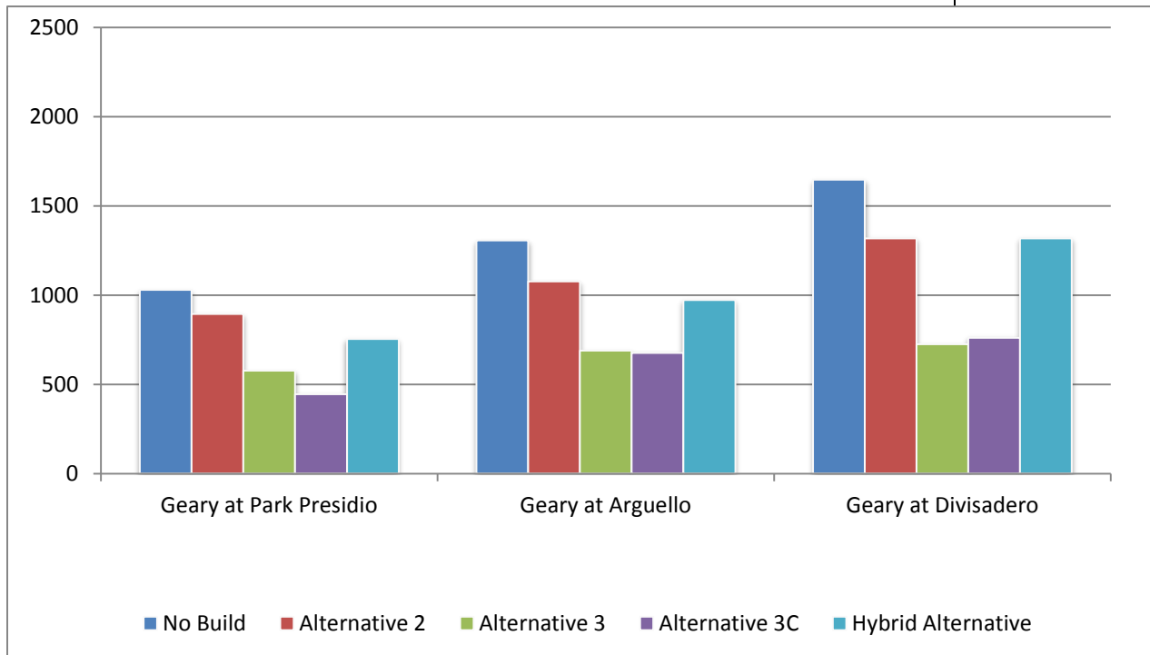
Figure 3.4-6 Geary Boulevard 2035 Eastbound PM P.M. Peak-Hour Traffic at Key Intersections (vehicles-Vehicles per hourHour)
