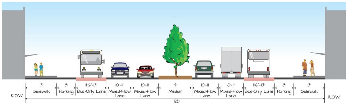
Figure 2-6 Figure 2-8 Proposed Cross-Section of Alternative 2 - Typical Section West of Gough Street
