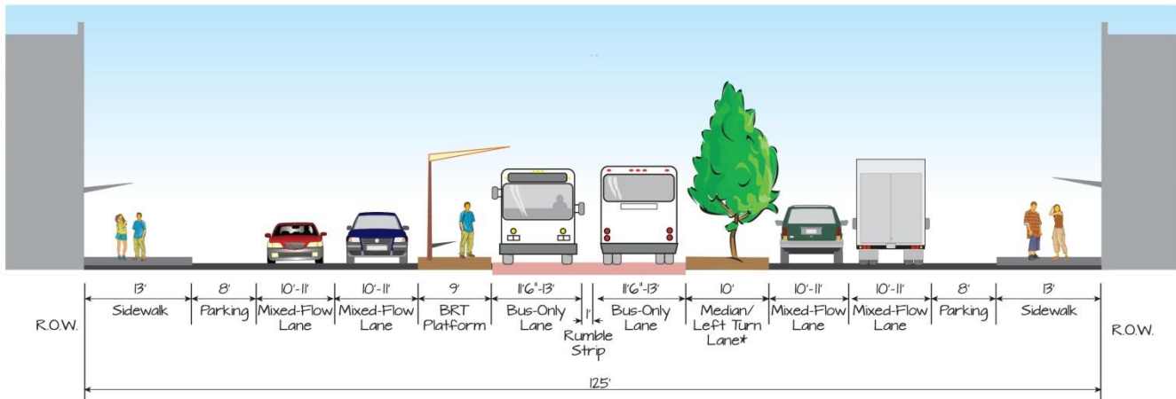
Figure 2-12 Figure 2-12 Figure 2-16 Figure 2-16 Proposed Cross-Section of Alternative 3-Consolidated
