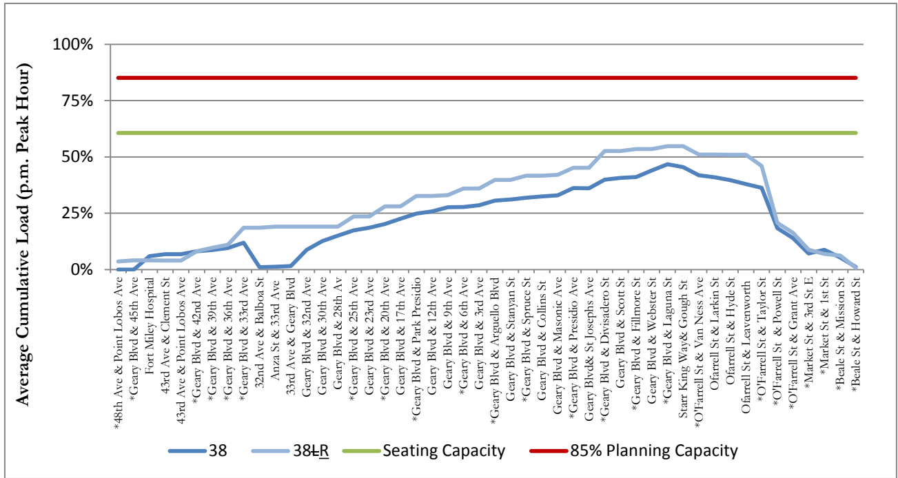
Figure 3.3-2 Average Load by Stop: Eastbound P.M. Peak Hour, 38 and 38LR
