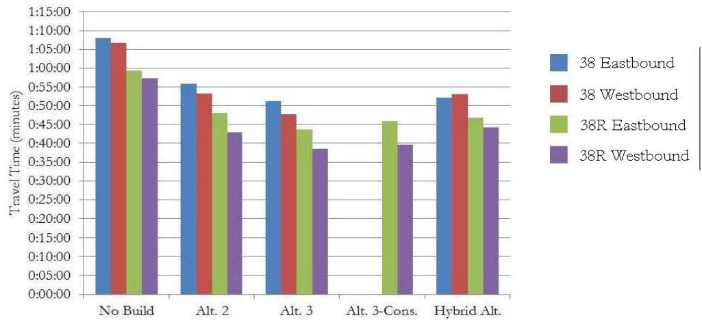
Figure 3.3-12 Year 2035 Geary Corridor Bus Travel Times (Entire Corridor, 48th Avenue to Transbay Terminal/Transbay Transit Center)
