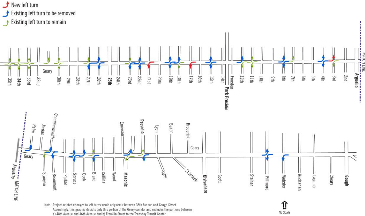
Figure 2-10 Figure 2-13 Proposed Left-Turn Locations for Alternative 3
