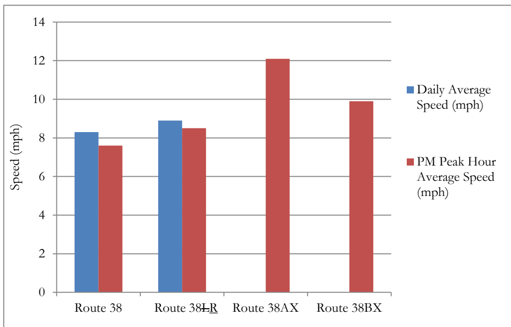
Figure 3.3-6 Existing Transit Speeds
