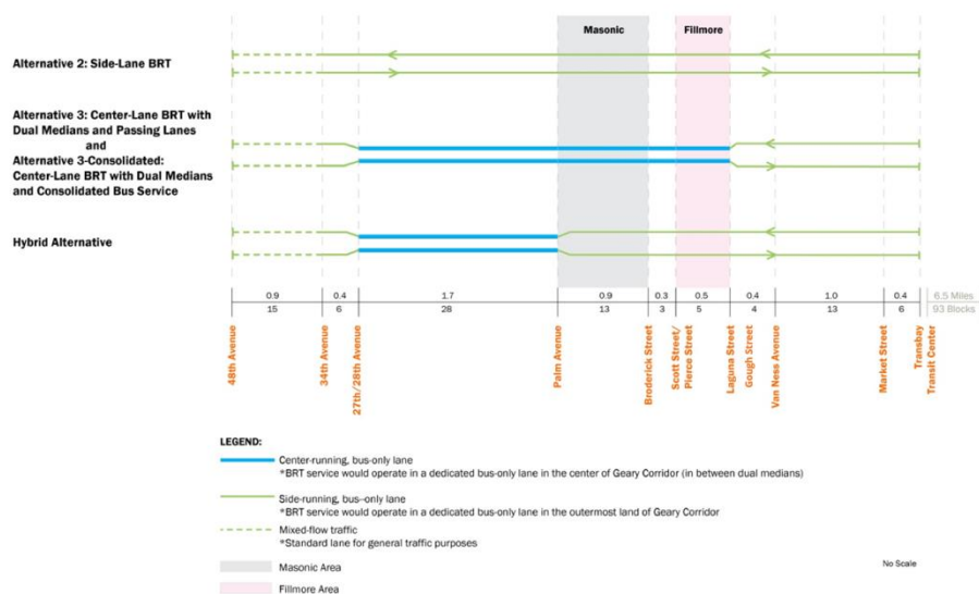
Figure S-1 Build Alternatives Schematic Diagram
