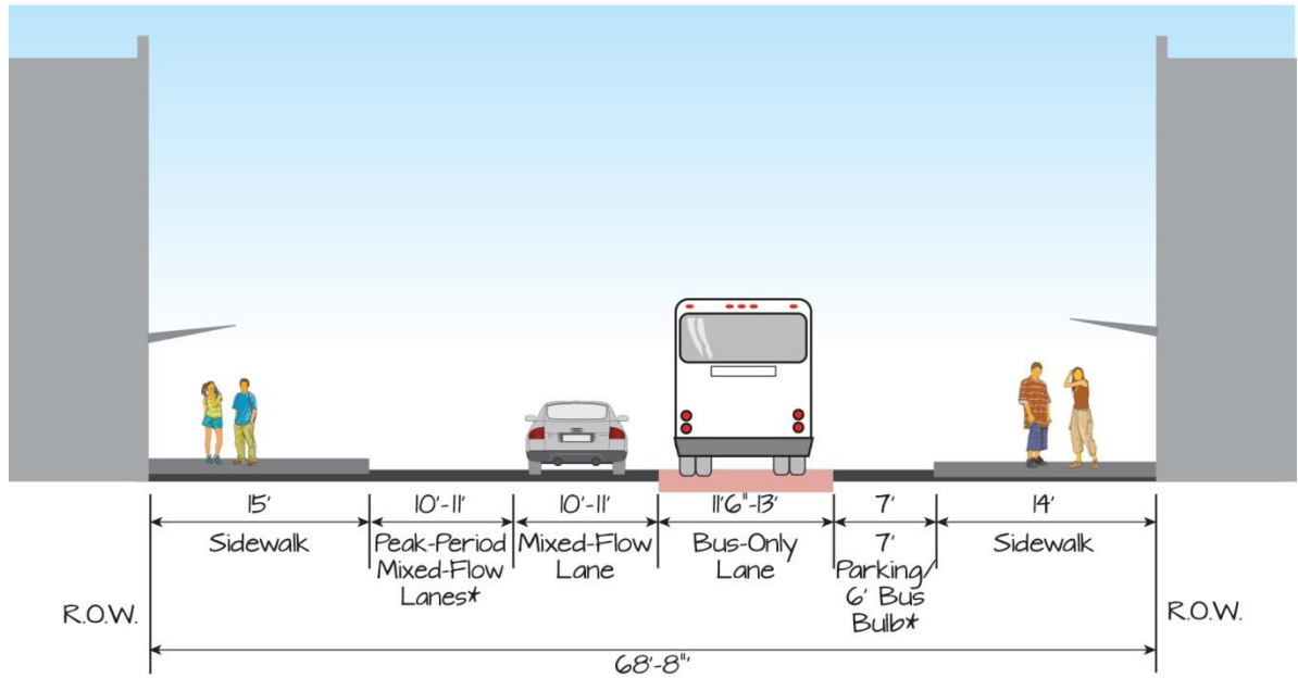
Figure 2-4 Figure 2-5 Proposed Cross-Section - East of Gough
