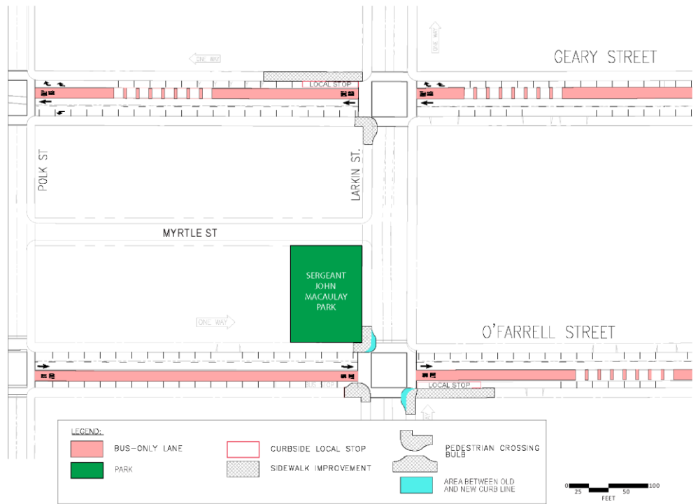
a) O'Farrell Street/Larkin Street Intersection without Additional Pedestrian Crossing Bulbs
