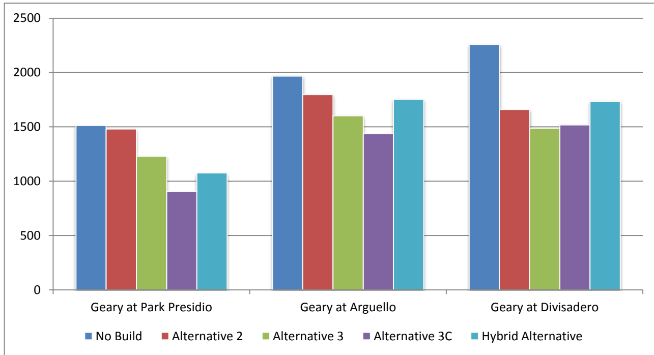
Figure 3.4-5 Geary Boulevard 2035 Westbound PM P.M. Peak-Hour Traffic at Key Intersections (vehicles-Vehicles per hourHour)
