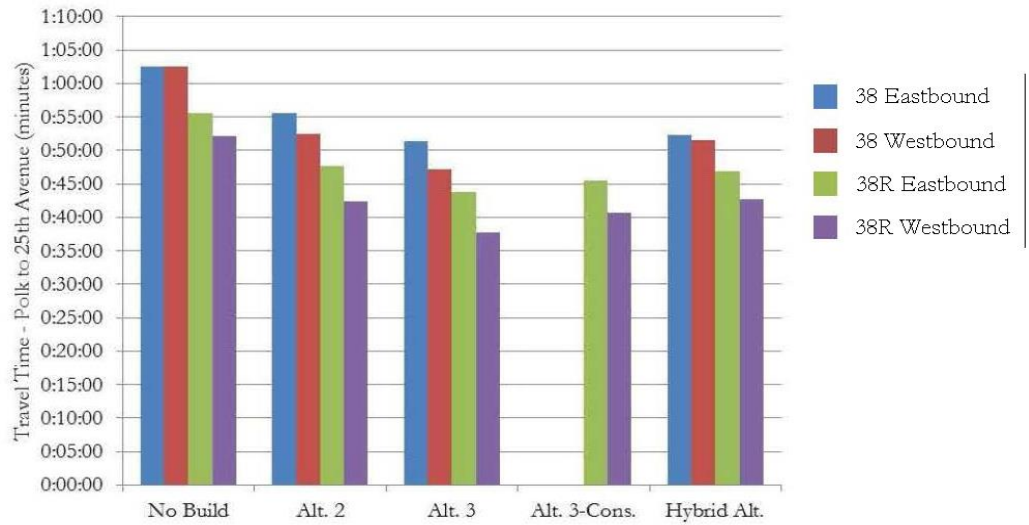
Figure 3.3-11 Year 2020 Geary Corridor Bus Travel Times (Entire Corridor, 48th Avenue to Transbay Terminal Transbay Transit Center)
