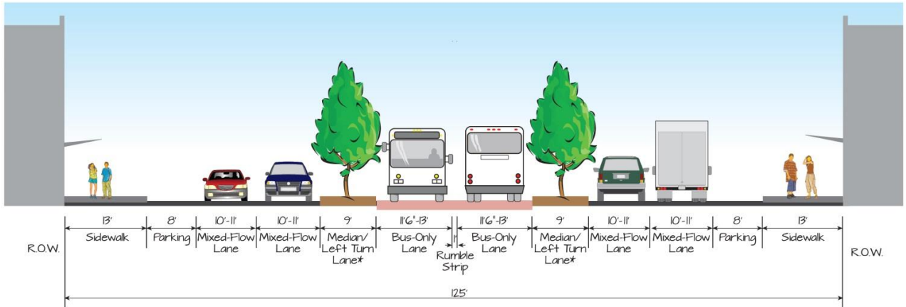
Figure 2-9 Figure 2-12 Proposed Typical Cross-Section of Alternative 3
