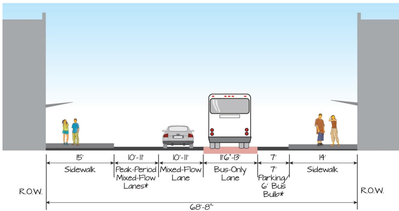
b) Typical Section East of Gough Street
