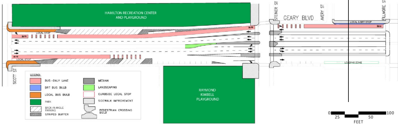
Figure 6-2 Geary Boulevard/Steiner Street Intersection (Hamilton Recreation Center and Raymond Kimbell Playground)
