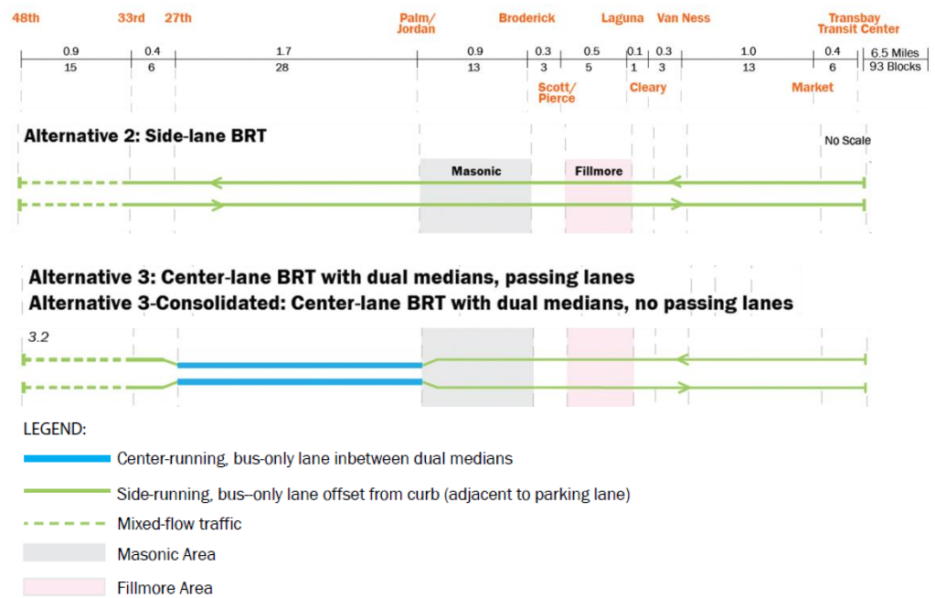
Figure 10-5 Remaining Alternatives and Combinations Under Consideration
