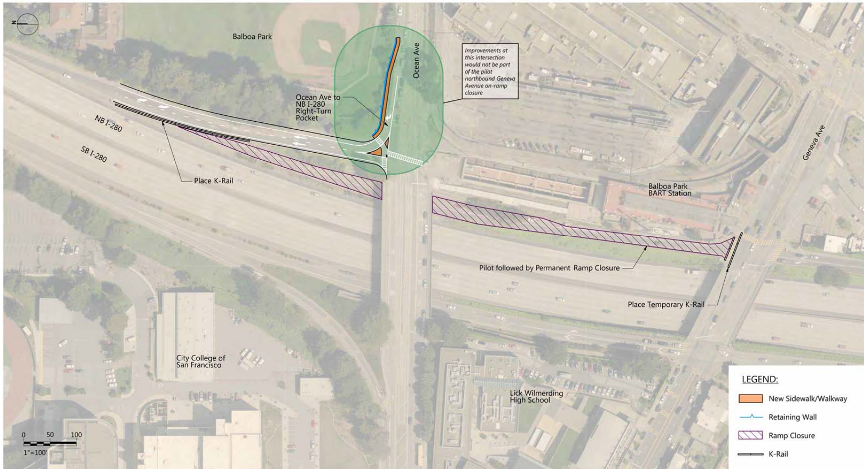
Figure 11: Alternative 1, Element 1 - Closure of Northbound Geneva On-Ramp and Re-Configuration of Northbound Ocean On-Ramp Intersection
