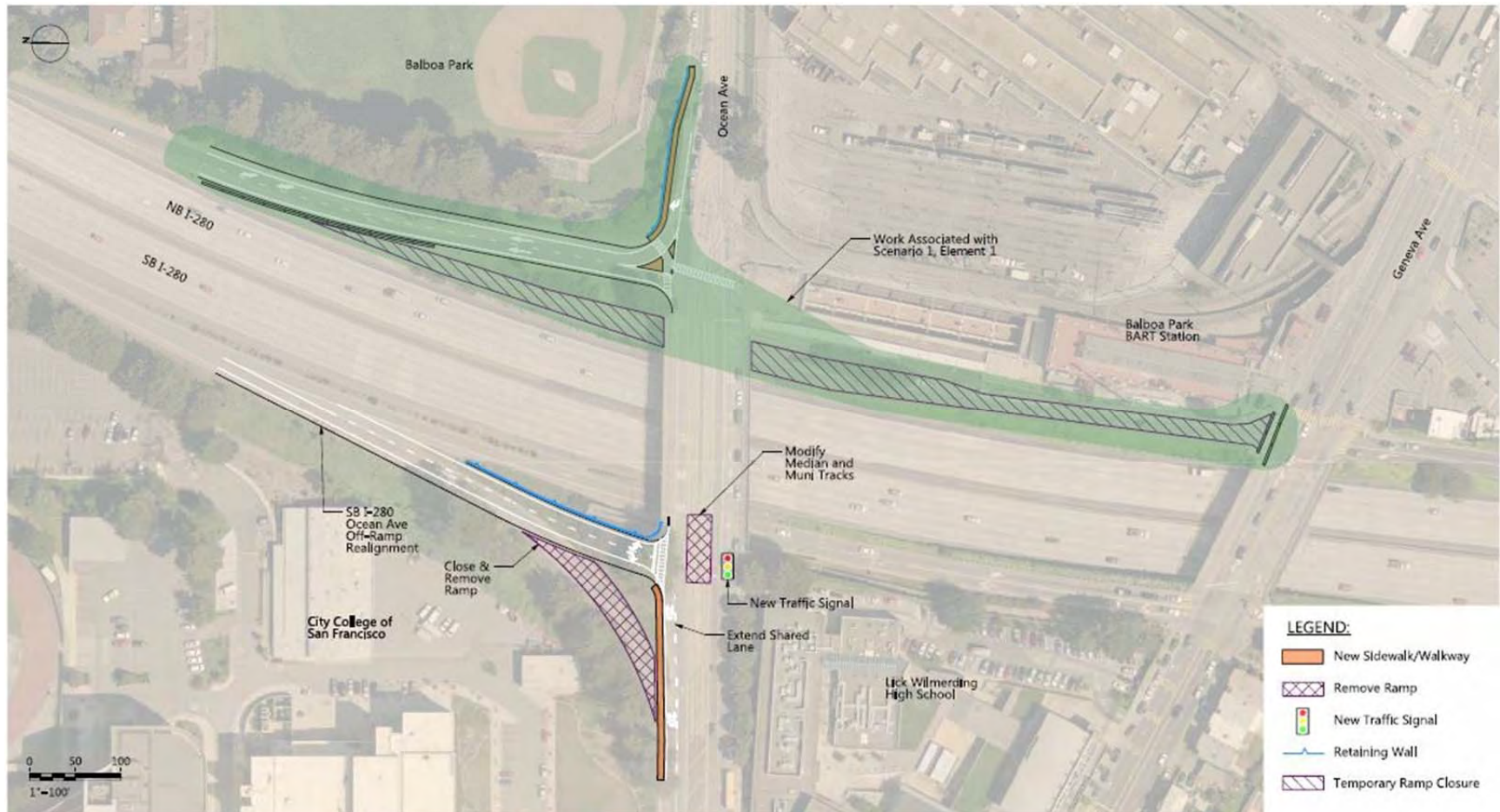
Figure 12: Alternative 1, Element 2 - Re-Configuration of Southbound Ocean Off-Ramp Intersection
