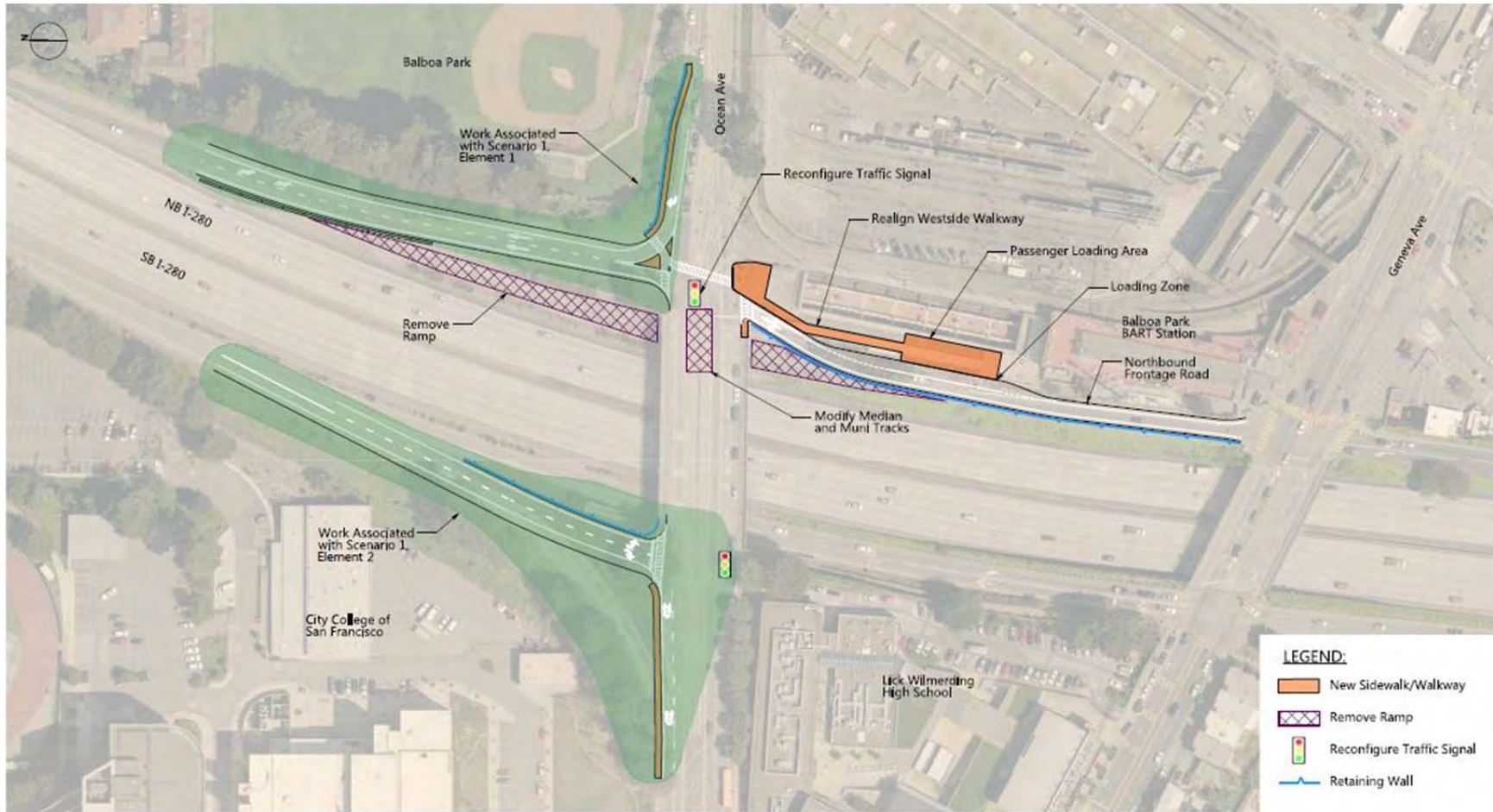
Figure 13: Alternative 1, Element 3 - Addition of New Northbound Kiss-And-Ride Frontage Road
