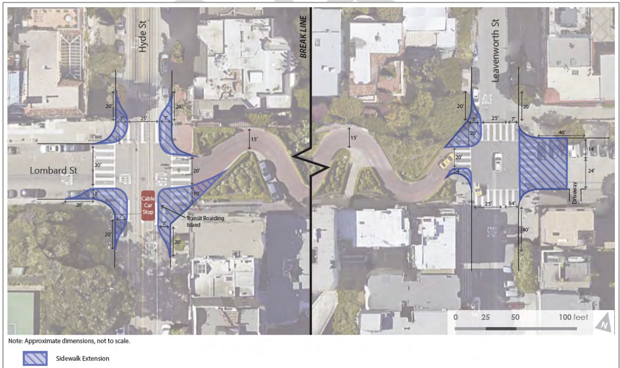
Figure 5. Conceptual Design 2 for Sidewalk Extensions (see appendix for full-size drawing)
