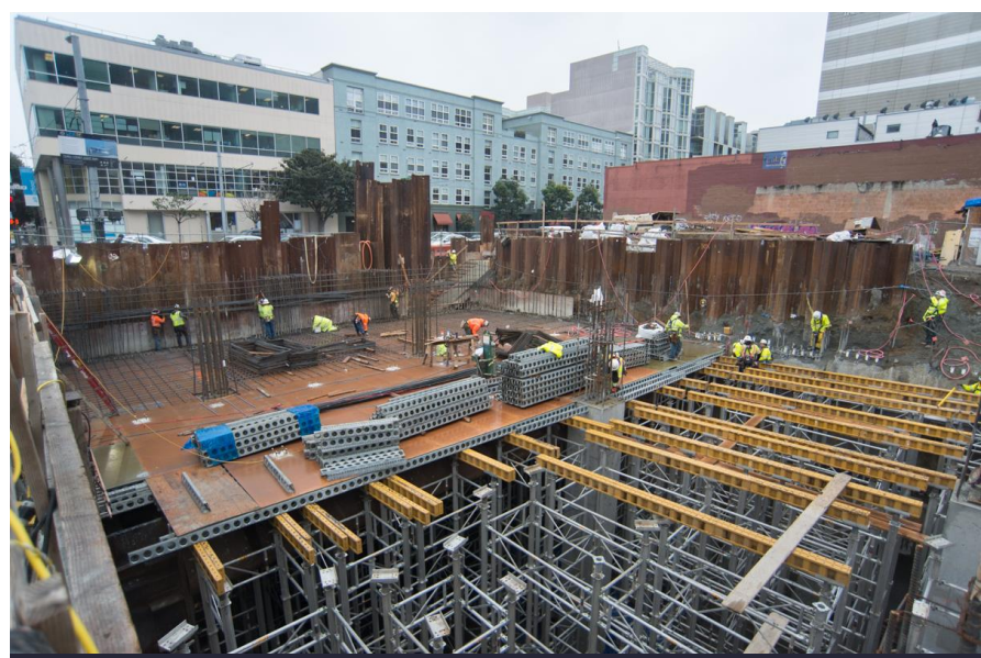
Various stages of roof deck construction can be seen inside the Yerba Buena/Moscone Station headhouse
