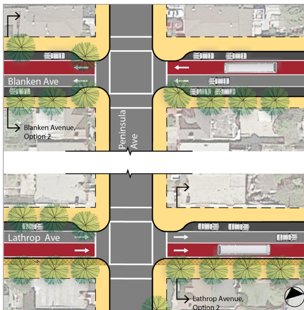
FIGURE 32. PLAN DRAWING OF BLANKEN/LATHROP COUPLET OPTION 2
